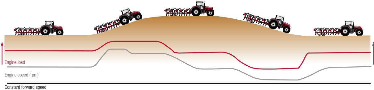
Dyna-TM: As the load (red line) varies according to the conditions, the Dyna-TM will automatically adjust the engine speed (grey line) to maintain the forward speed whilst minimising fuel consumption and noise levels.
